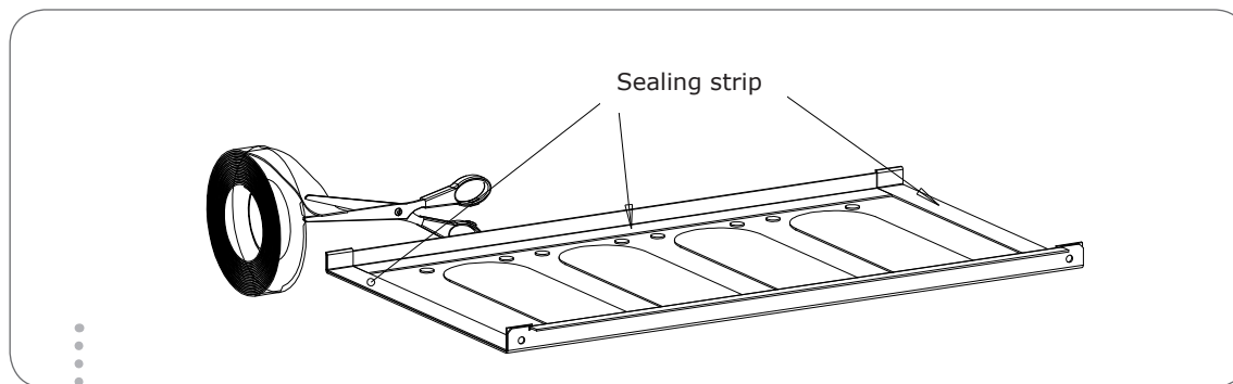
Fig. 3.3 Sealing of end plates. Sealing strip is attached to the short sides of end plates.
