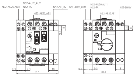
Figure 5 Assembly positions and dimensions of accessories
