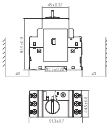
Figure 4 Overall and installation dimensions of NS2-32H
