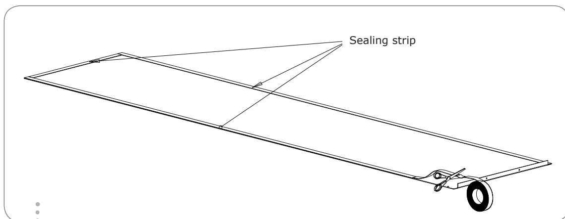
Fig. 3.2 Sealing long sides and lower side of back plate for F-series cell centre with sealing strip (50020040 Joint sealing strip 0.8*20 mm).
