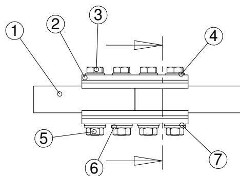
Fig 10.4. Connecting of busbars at a transport break. The busbars are connected using connecting pieces of aluminium (e.g. YKG 51/120), M10 screws and nuts, and various washers.
