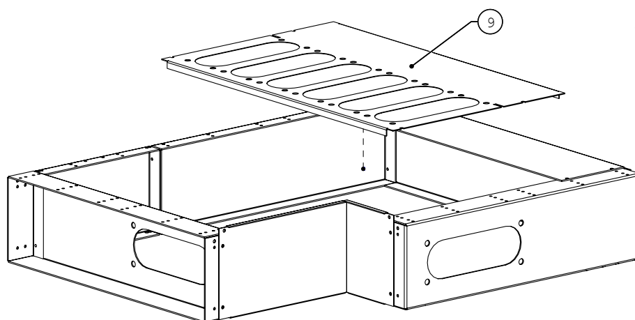
Fig 2.21 Attach base plate (9) to base intermediate plate (10) and base end plate (12).
