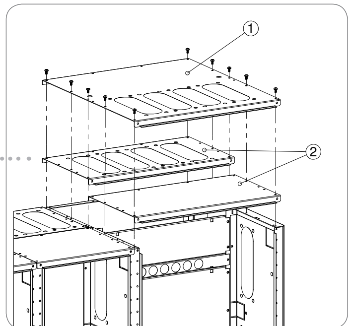
Fig. 2.6 Top cover alternatives of the F-serie system. The top cover can be made using either a single, full-depth end plate or two 250 mm deep end plates (2).
