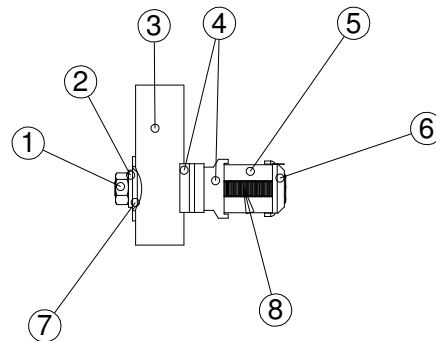
Fig 10.3. Connecting vertical and horizontal busbars using YKG busbar connectors.
