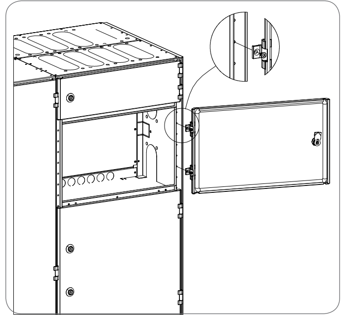
Fig. 2.17 Mounting doors to frame structure. Doors are fastened with screws to side plate or front profile.
