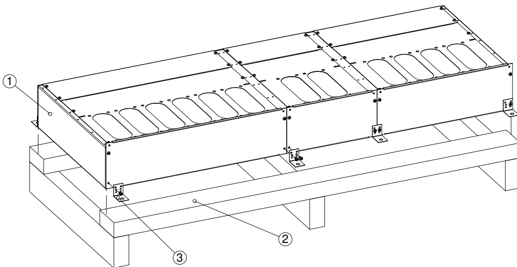
Fig. 2.2 Base and wooden base frame. The base (1) is fastened to the wooden base frame (2) using base fastening brackets (3).
