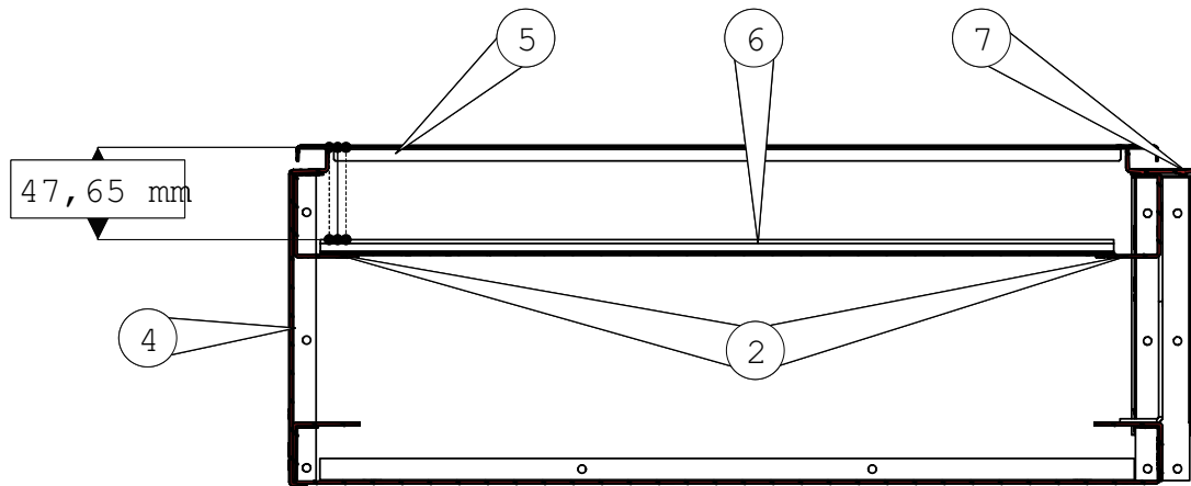
Fig 8.7.3 Sectional view. The distance between DIN rail (6) surface and the back of the cover is 47.65mm.
