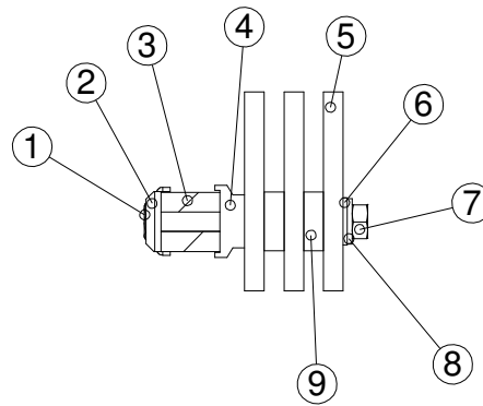
Fig 10.2. Connecting feed and horizontal power busbars together.
