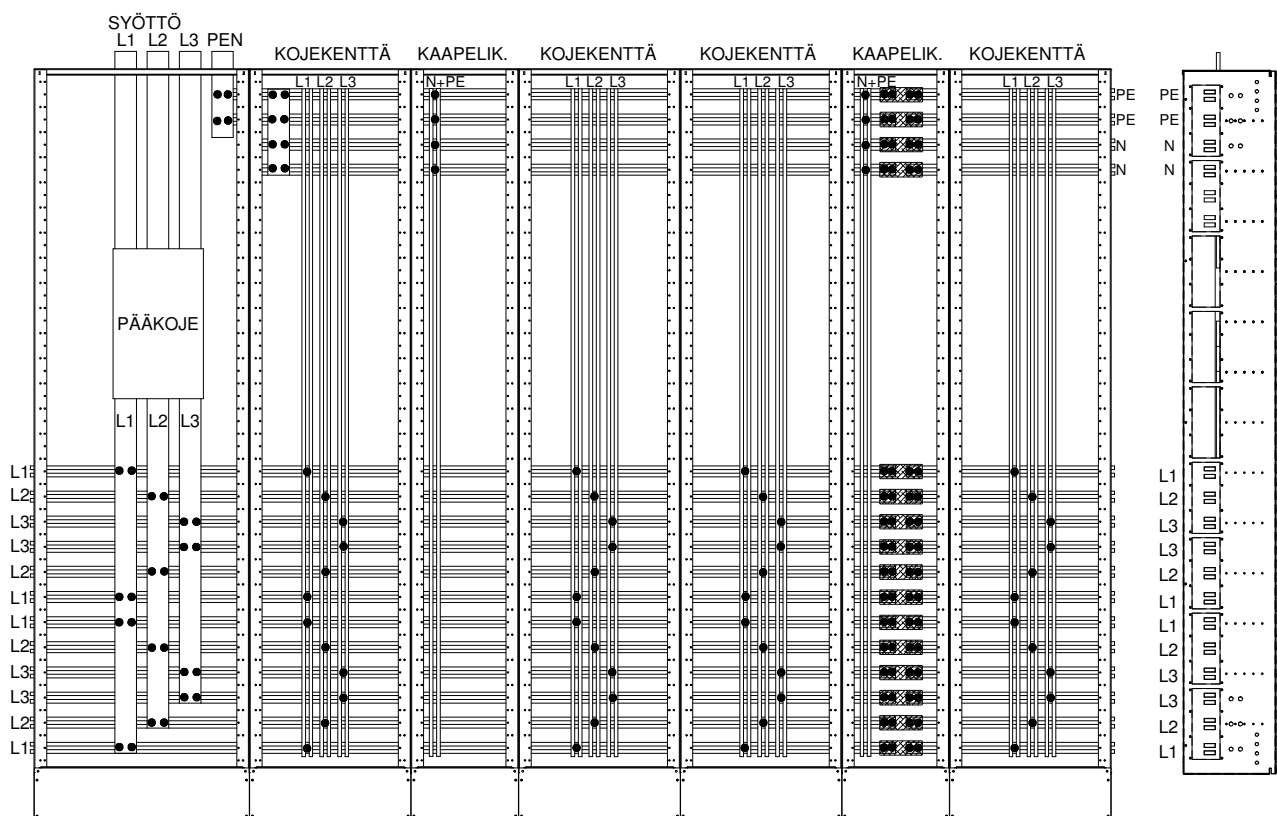
Fig. 4.2 An example of busbar system and installation arrangement in an F-series cell centre. Black dots (•) indicate busbar connections.
