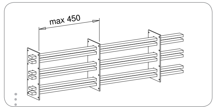
Fig 4.1 In F-series system the insulator distance may not exceed 450 mm.
