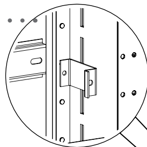
Fig 8.7.4 Spacers are fastened to back plates, and DIN rails to spacers.
