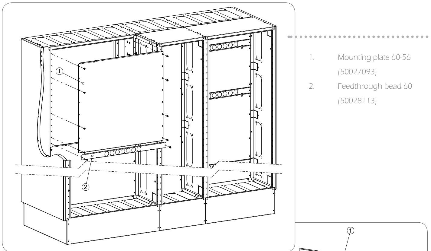
Fig. 2.12. Fastening mounting plates and feedthrough beads to frame structure. Feedthrough beads restrict the spreading of arc from busbar space to component space in the cell centre.
