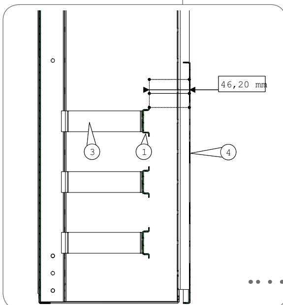
Fig 8.7.5 Sectional view of spacers and DIN rails. The distance between DIN rail surface and the back of the cover is 46.2 mm.
