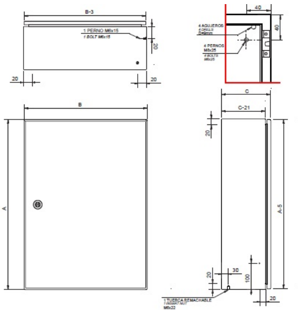
Standard drawing
