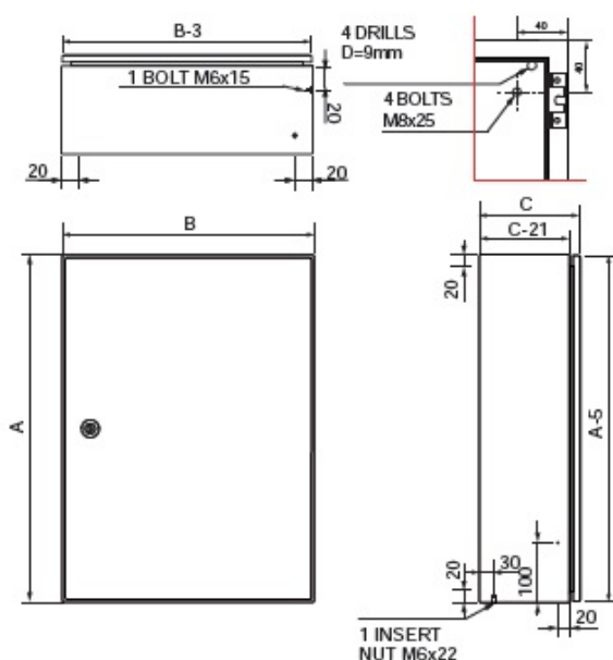
Standard drawing
