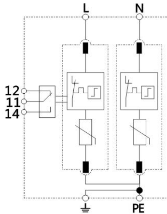
Electrical principle
