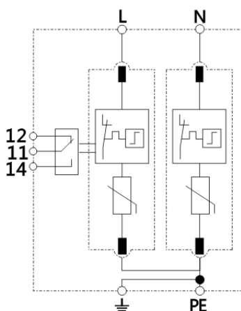
Electrical principle
