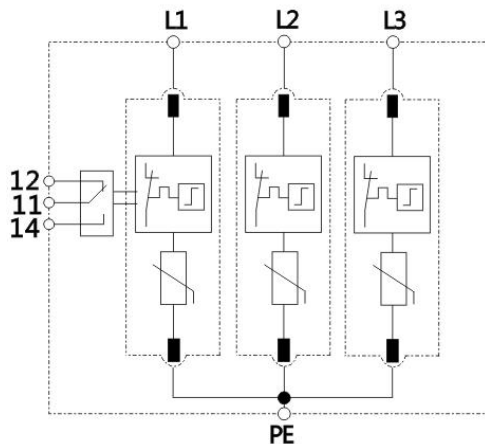
Electrical principle
