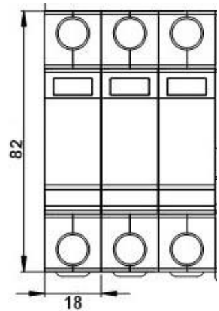
Outline dimension
