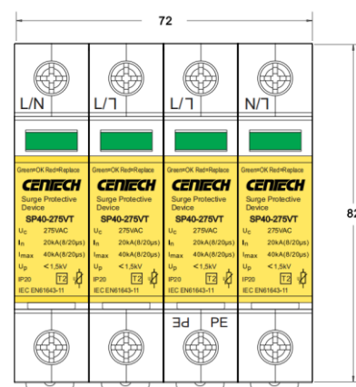
Outline dimension
