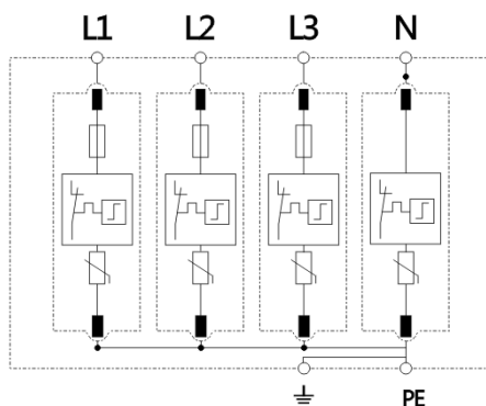
Electrical principle
