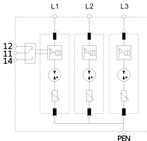
Electrical principle
