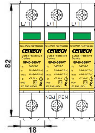
Outline dimension
