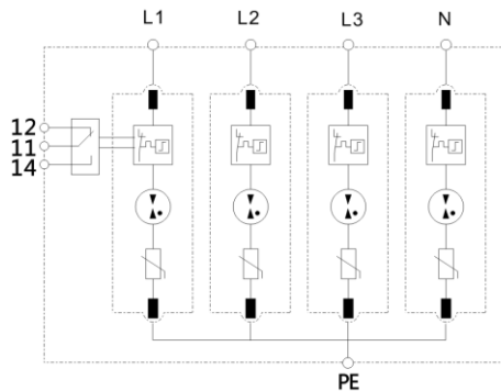
Electrical principle
