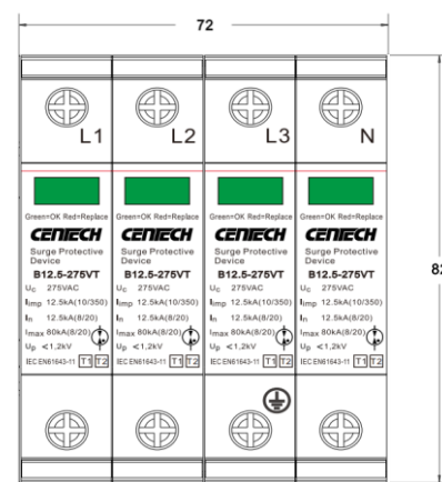
Dimension drawing
