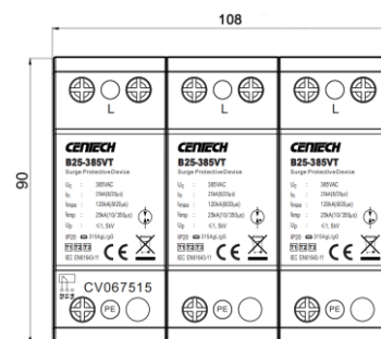
Dimension drawing
