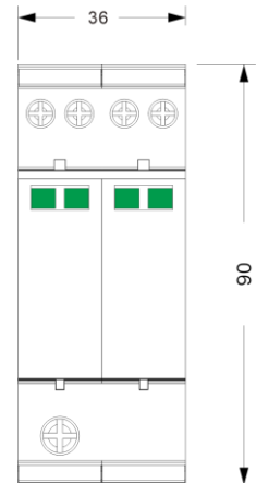
Outline dimension
