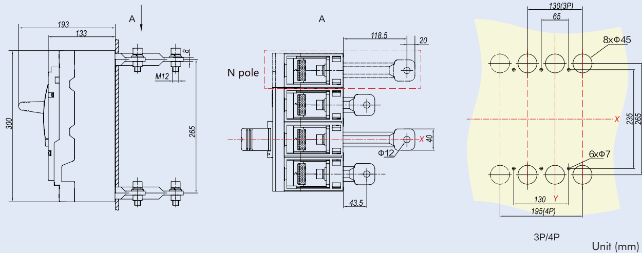
NM8N-800 Rear connection
