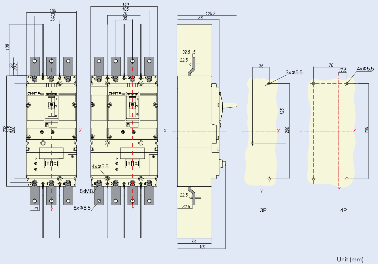
NM8NL-250 Front connection
