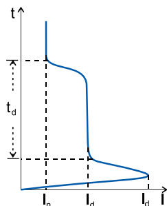
Motor starting Current curve
