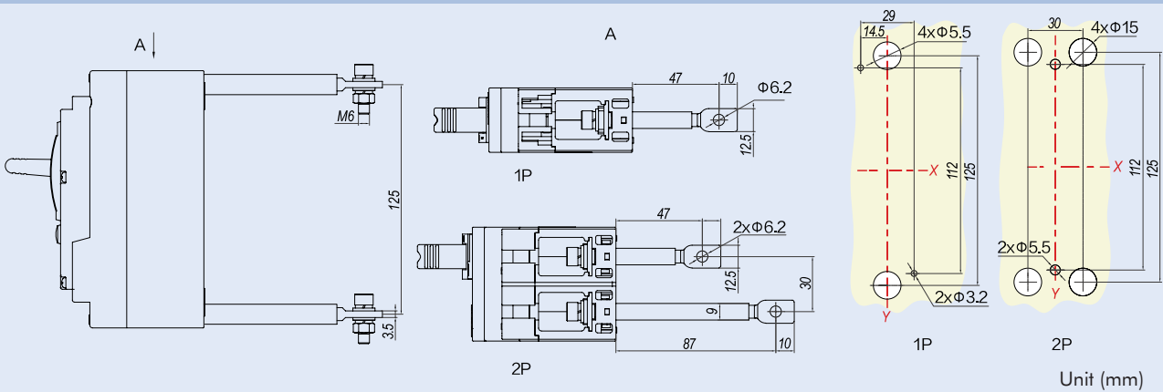
NM8N-125 Rear connection (1P/2P)
