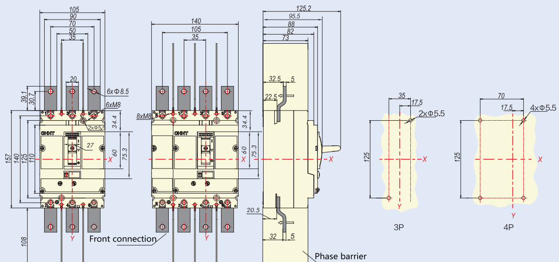
NM8N-250 Front connection (3P/4P)
