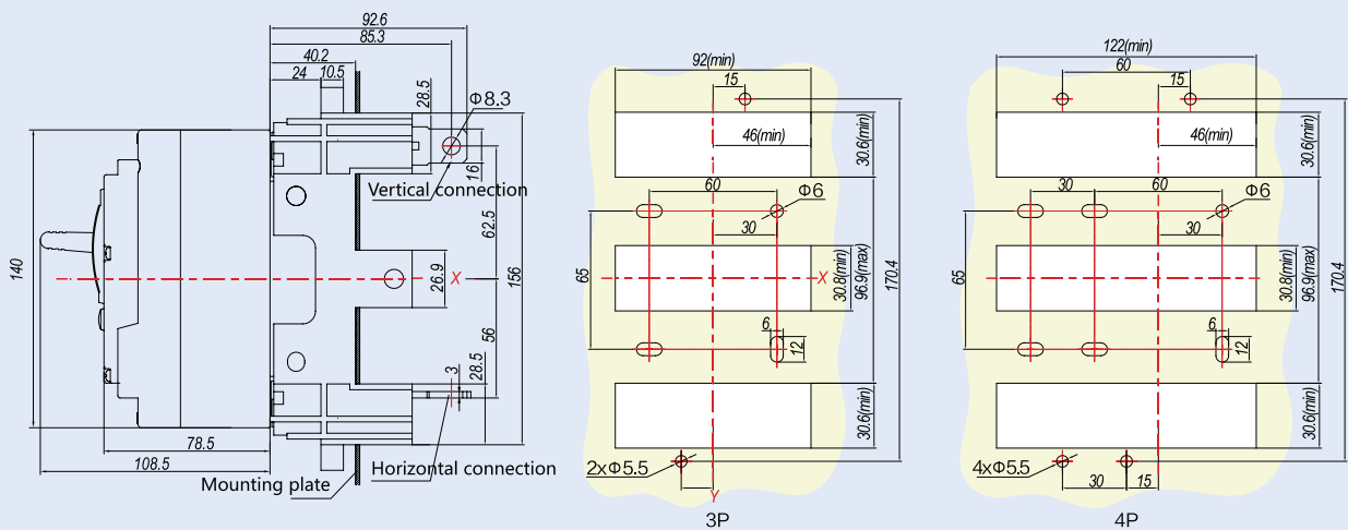
NM8N-125 Plug-in rear connection
