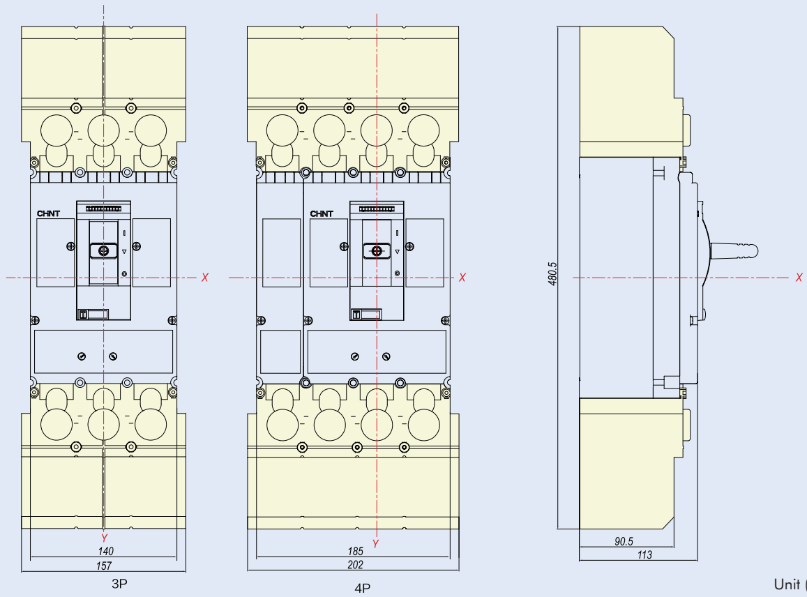
NM8N-400/630 Long terminal cover
