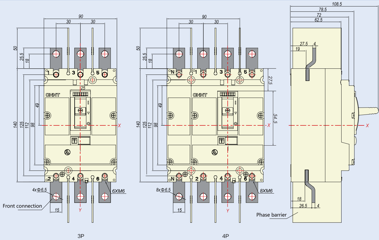
NM8N-125 Front connection (3P/4P)
