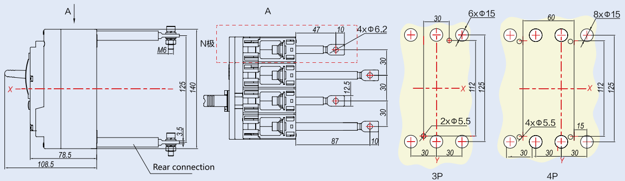
NM8N-125 Rear connection (3P/4P)
