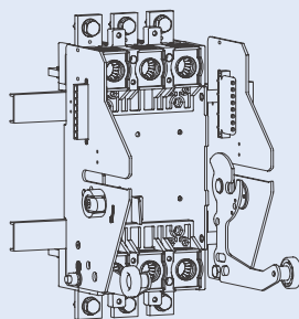
DIN-rail mounting
