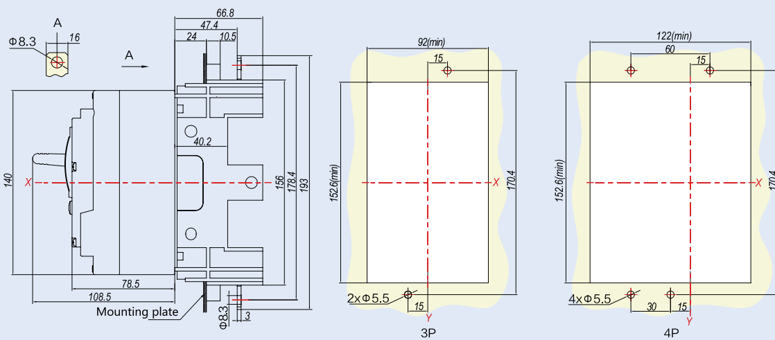
NM8N-125 Plug-in front connection
