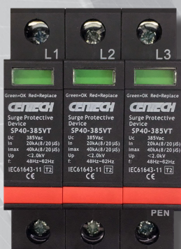
OVERSPENNINGSVERN 3-POL (385V)
